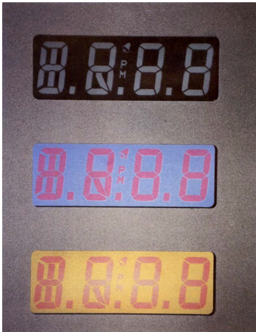
FIGURE 7 Reflective phase-change guest-host display operated at 5.5 volts containing black-white mixture G; no polarizers used (first display from the top). Reflective nematic L/T-displays with parallel wall alignment operated at 4.5 volts containing RO-TN-605 as a host (second and third display from the top). One polarizer aligned parallel to the back wall alignment was used in front of the reflector of the L/T-displays.
